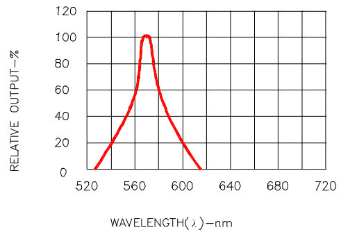
Fig.2 SPECTRAL RESPONSE
