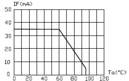
Maximum Forward DC Current vs Ambient Temperature
