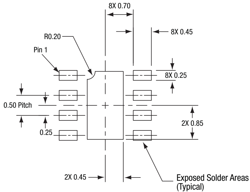
Figure 31. SKY67021-396LF PCB Layout Footprint (Top View)
